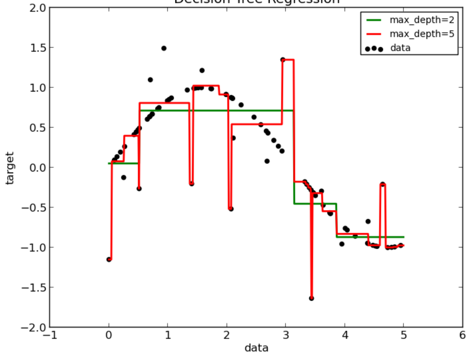
Decision Tree Regression
